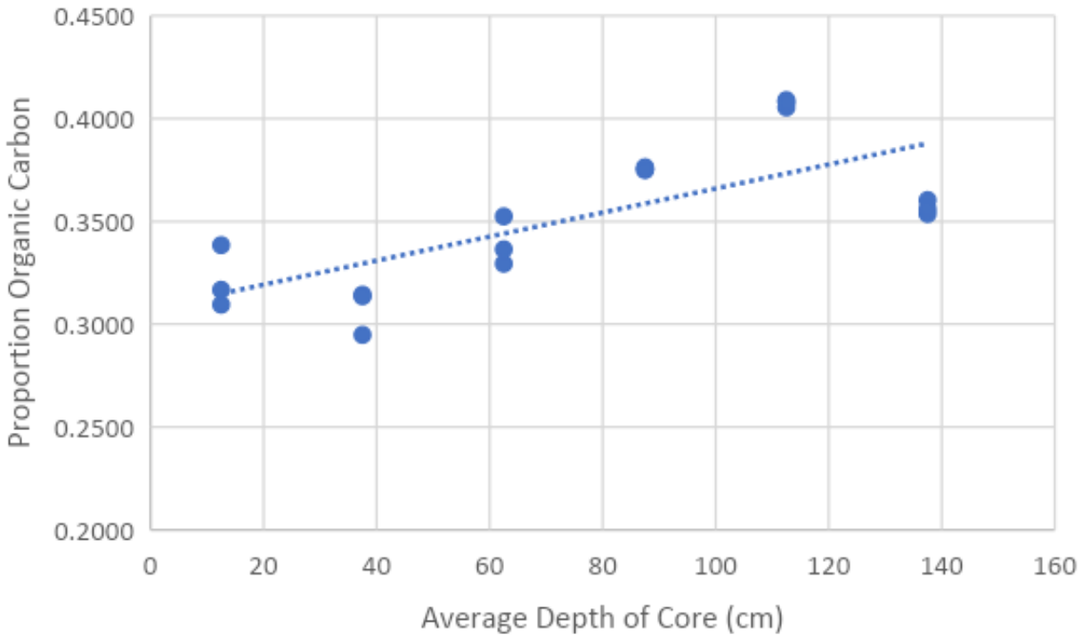
Figure 21. Proportion organic carbon for core subsections from different depths in a low shrub peatland near Kachemak Dr in Homer, AK. Organic carbon mostly increases with depth; measured peat depth near this location was 178 cm, so the deepest sample is relatively close to the bottom of the peat.
